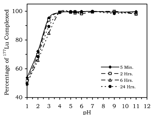
Figure 6. Complex Lu(NP-DO3A) is stable over the pH range 4–11 for up to 24 h, with greater than 98% of the complex remaining intact in this pH range. Dissociation of the complex is only observed at pH 3 or below.
