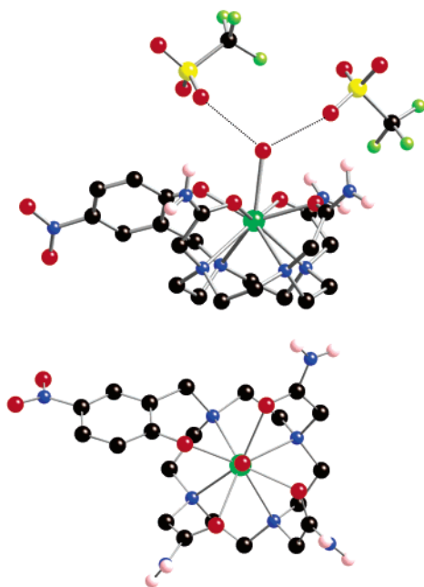
Figure 1. Crystal structure of Eu(NP-DO3AM)(H 2 O)(CF 3 SO 2 - ) 2 showing a side view (upper) and top view (lower). Hydrogen atoms bonded to carbon have been omitted for clarity. The structure shown is the \Delta(\lambda\lambda\lambda\lambda) conformer, the \Lambda(\delta\delta\delta\delta) conformer, cocrystallized in the P \bar{1} unit cell, is not shown. The dotted lines indicate the hydrogen-bonding interactions of the coordinated water molecule and the triflate anions. An ORTEP rendering of the structure is included in the ESI.
